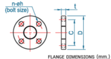
FLANGE DIMENSIONS (mm.)
